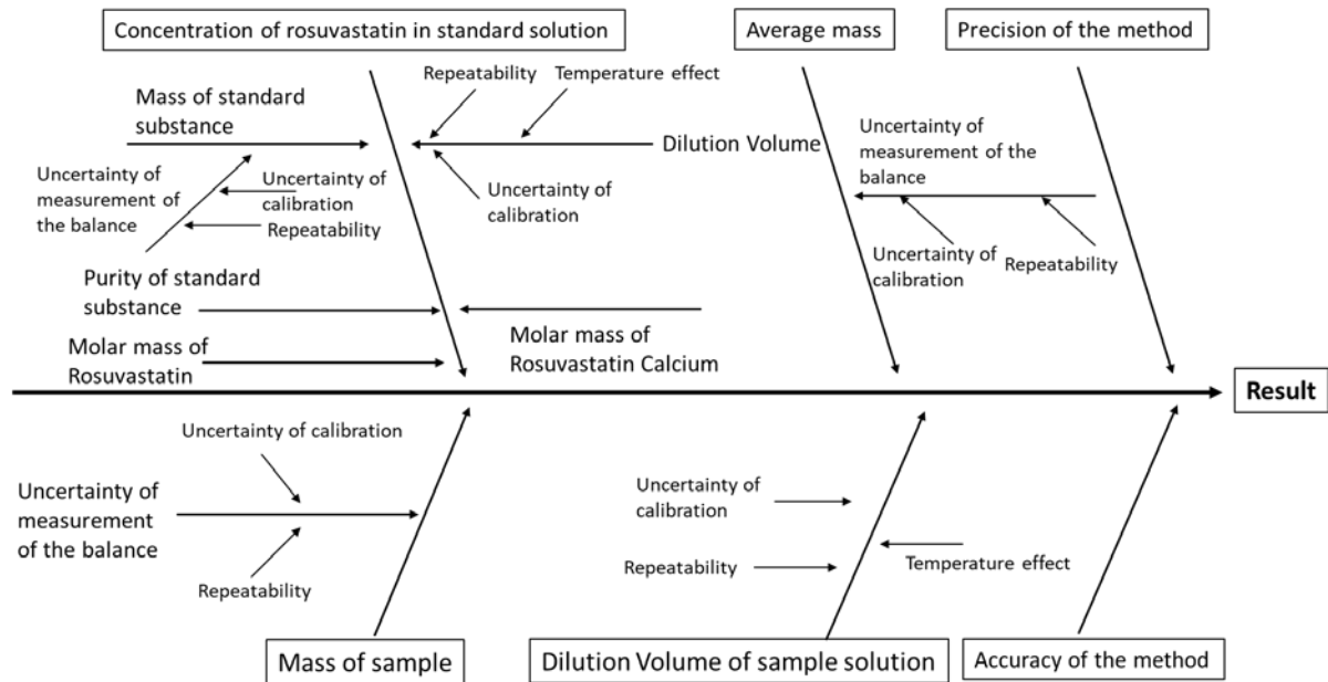
Fig. 1 Cause and effect diagram for HPLC determination of content of Rosuvastatin
