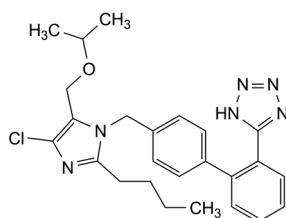
F. 5-[4'-[[2-butyl-4-chloro-5-[[1-(1-methylethyl)oxy]methyl]-1H-imidazol-1-yl]methyl]biphenyl-2-yl]-1H-tetrazole,
