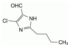
D. 2-butyl-4-chloro-1H-imidazole-5-carbaldehyde,
