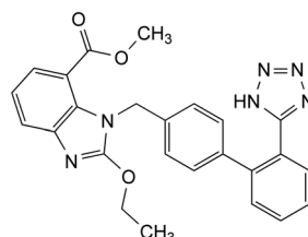
I. methyl 2-ethoxy-1-[[2'-(1 H -tetrazol-5-yl)biphenyl-4-yl]methyl]-1 H -benzimidazole-7-carboxylate.
