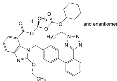
F. (1 RS )-1-[[[(cyclohexyloxy)carbonyl]oxy]ethyl] 2-ethoxy-1-[[2'-(2-ethyl-2 H -tetrazol-5-yl)biphenyl-4-yl]methyl]-1 H -benzimidazole-7-carboxylate,
