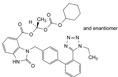
C. (1 RS )-1-[[[(cyclohexyloxy)carbonyl]oxy]ethyl] 3-[[2'-(1-ethyl-1 H -tetrazol-5-yl)biphenyl-4-yl]methyl]-2-oxo-2,3-dihydro-1 H -benzimidazole-4-carboxylate,
