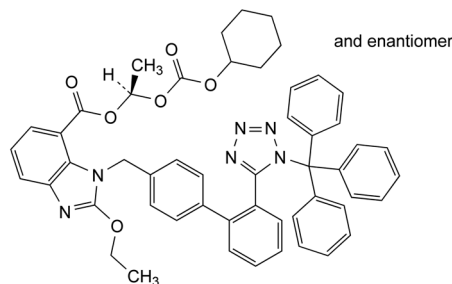
H. (1 RS )-1-[[[(cyclohexyloxy)carbonyl]oxy]ethyl] 2-ethoxy-1-[[2'-[1-(triphenylmethyl)-1 H -tetrazol-5-yl]biphenyl-4-yl]methyl]-1 H -benzimidazole-7-carboxylate ( N -tritylcandesartan),
