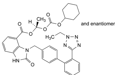
D. (1 RS )-1-[[[(cyclohexyloxy)carbonyl]oxy]ethyl] 3-[[2'-(2-ethyl-2 H -tetrazol-5-yl)biphenyl-4-yl]methyl]-2-oxo-2,3-dihydro-1 H -benzimidazole-4-carboxylate,
