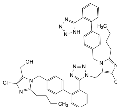
L. [2-butyl-1-[[2'-[1-[[2-butyl-4-chloro-1-[[2'-(1H-tetrazol-5-yl)biphenyl-4-yl]methyl]-1H-imidazol-5-yl]methyl]-1H-tetrazol-5-yl]biphenyl-4-yl]methyl]-4-chloro-1H-imidazol-5-yl]methanol,
