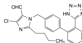
K. 2-butyl-4-chloro-1-[[2'-(1H-tetrazol-5-yl)biphenyl-4-yl]methyl]-1H-imidazol-5-carbaldehyde,
