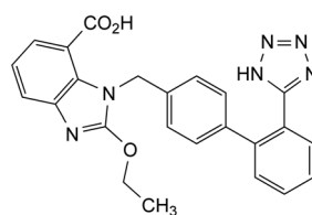
G. 2-ethoxy-1-[[2'-(1 H -tetrazol-5-yl)biphenyl-4-yl]methyl]-1 H -benzimidazole-7-carboxylic acid (candesartan),
