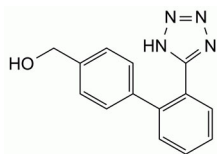
B. [2'-(1H-tetrazol-5-yl)biphenyl-4-yl]methanol,
