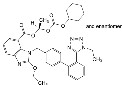
E. (1 RS )-1-[[[(cyclohexyloxy)carbonyl]oxy]ethyl] 2-ethoxy-1-[[2'-(1-ethyl-1 H -tetrazol-5-yl)biphenyl-4-yl]methyl]-1 H -benzimidazole-7-carboxylate,
