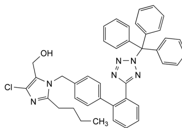
H. [2-butyl-4-chloro-1-[[2'-(2-(triphenylmethyl)-2H-tetrazol-5-yl)biphenyl-4-yl]methyl]-1H-imidazol-5-yl]methanol,
