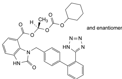
B. (1 RS )-1-[[[(cyclohexyloxy)carbonyl]oxy]ethyl] 2-oxo-3-[[2'-(1 H -tetrazol-5-yl)biphenyl-4-yl]methyl]-2,3-dihydro-1 H -benzimidazole-4-carboxylate,
