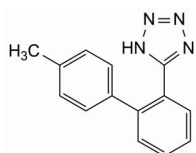
E. 5-(4'-methylbiphenyl-2-yl)-1H-tetrazole,
