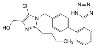
C. [2-butyl-5-chloro-1-[[2'-(1H-tetrazol-5-yl)biphenyl-4-yl]methyl]-1H-imidazol-4-yl]methanol,
