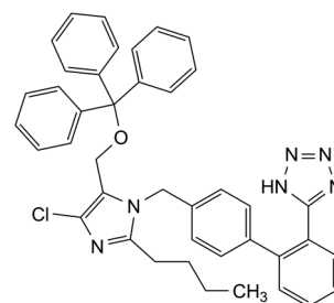
I. 5-[4'-[[2-butyl-4-chloro-5-[[1-(triphenylmethyl)oxy]methyl]-1H-imidazol-1-yl]methyl]biphenyl-2-yl]-1H-tetrazole,
