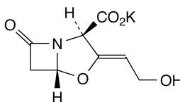
45 46 Figure A-4-1. – Potassium clavulanate, diluted (1653)
