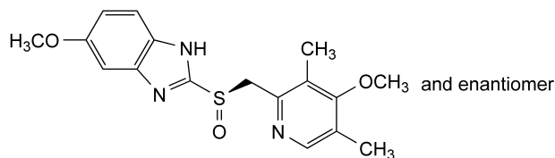
10 Figure A-7-12. – Omeprazole (0942)
