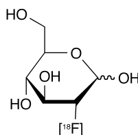
44 Figure A-5-2. – Fludeoxyglucose ( 18 F) injection (1325)
