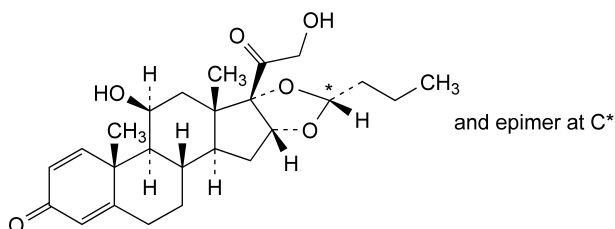
Figure A-7-17. – Budesonide (1075)
