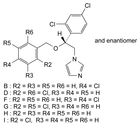
28 29 Figure FAQ-7. – Impurities B, D, F, G, H and I of Miconazole nitrate (0513)
