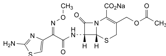
Figure A-7-5. – Cefotaxime sodium (0989)
