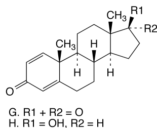
8 9 Figure FAQ-6. – Impurities G to H of Testosterone (1373)
