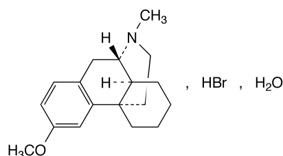
7 8 Figure A-4-15. – Dextromethorphan hydrobromide (0020)
