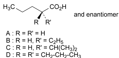
42 43 44 Figure FAQ-8. – Impurities A to D of Valproic acid (1378)
